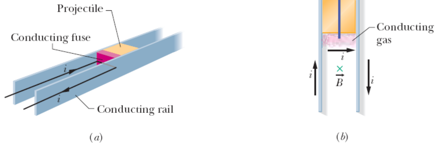
Fig. 29-10 (a) A rail gun, as a current i is set up in it. The current rapidly causes the conducting fuse to vaporize. (b) The current produces a magnetic field \vec{B} between the rails, and the field causes a force \vec{F} to act on the conducting gas, which is part of the current path. The gas propels the projectile along the rails, launching it.
