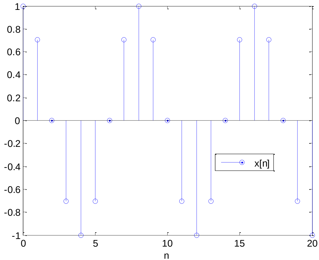
Fig. 7.8: Discrete-time sinusoid
