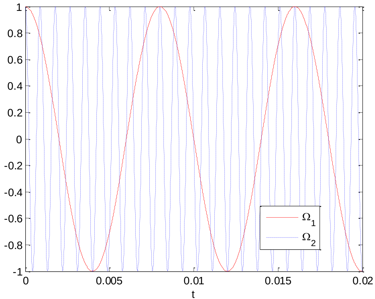
Fig. 7.9: Continuous-time sinusoids
