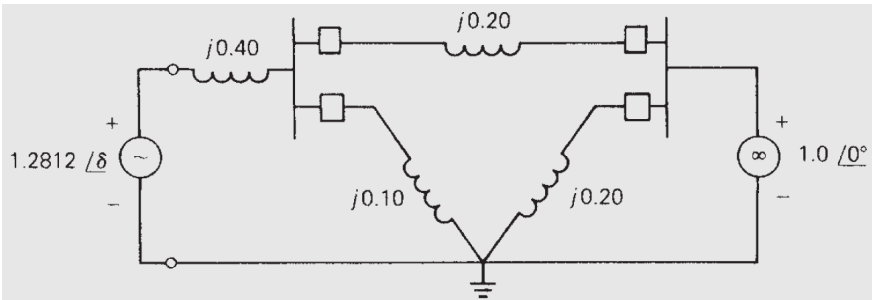
Faulted network
