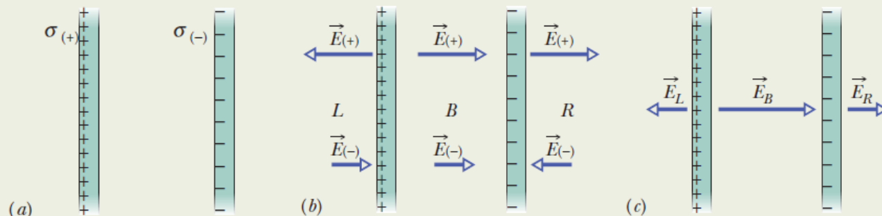
Fig. 23-17 (a) Two large, parallel sheets, uniformly charged on one side. (b) The individual electric fields resulting from the two charged sheets. (c) The net field due to both charged sheets, found by superposition.
