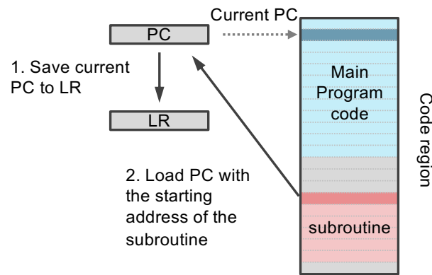
Call a subroutine
