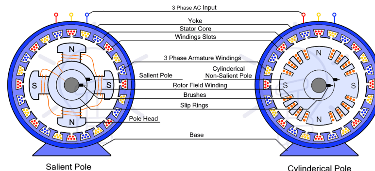
Construction of Synchronous Motor
