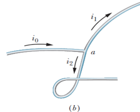
Fig. 26-3 The relation i_0 = i_1 + i_2 is true at junction a no matter what the orientation in space of the three wires. Currents are scalars, not vectors.
